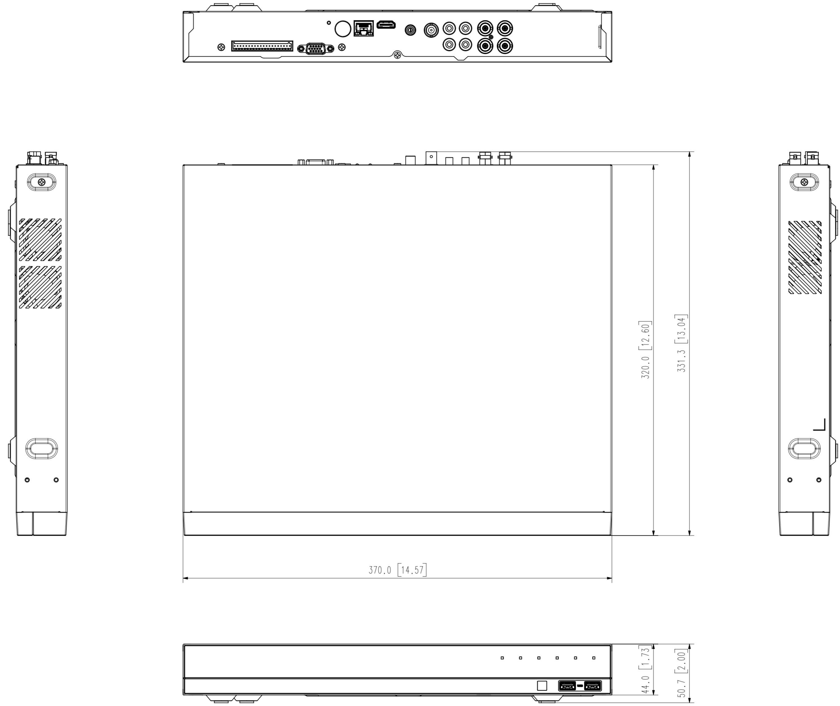
Appearance drawing HRX-421 Unit : mm[inches]
