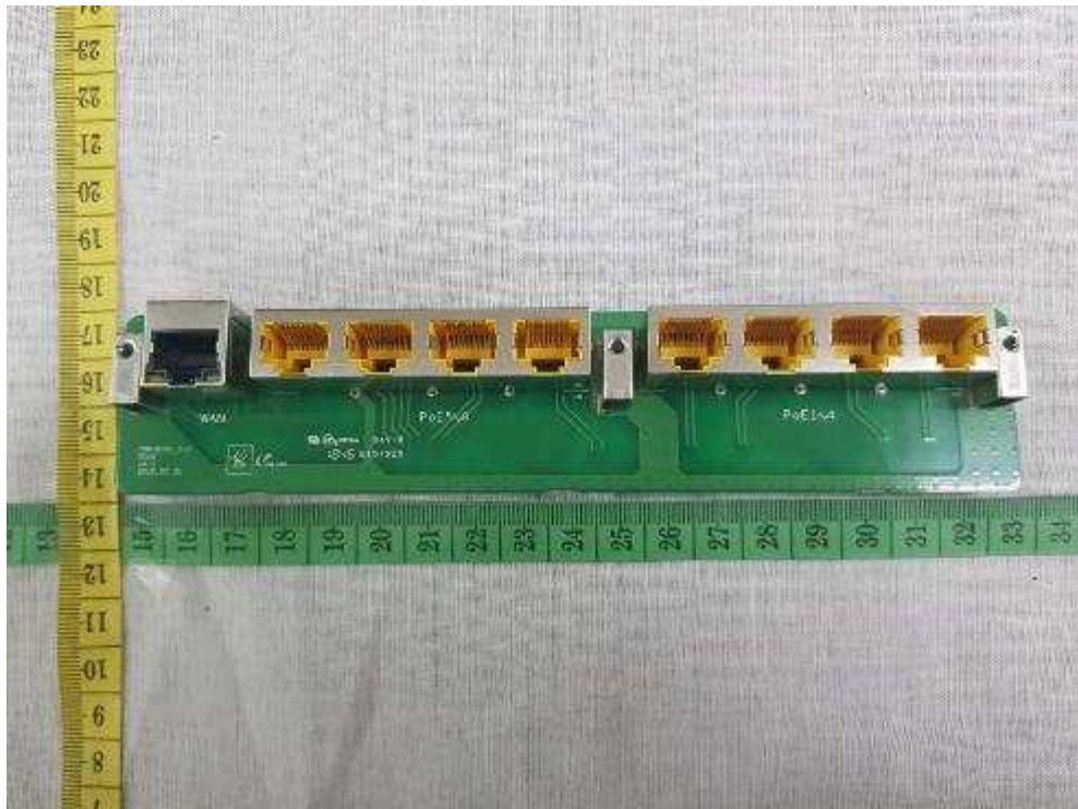
< PoE PCB top view >
